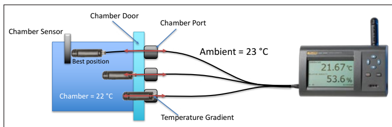
Figure 3. Example of proper DUT placement to reduce uncertainty due to non-uniformity and stem effect
