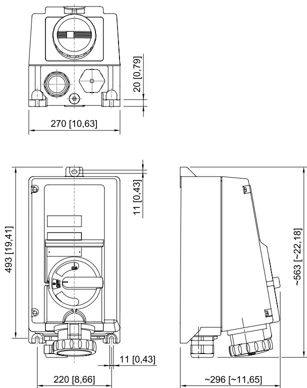
Wall-mounting socket
