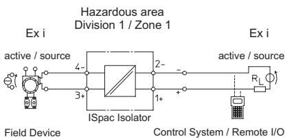
Connection diagram 9164/13-20-08
