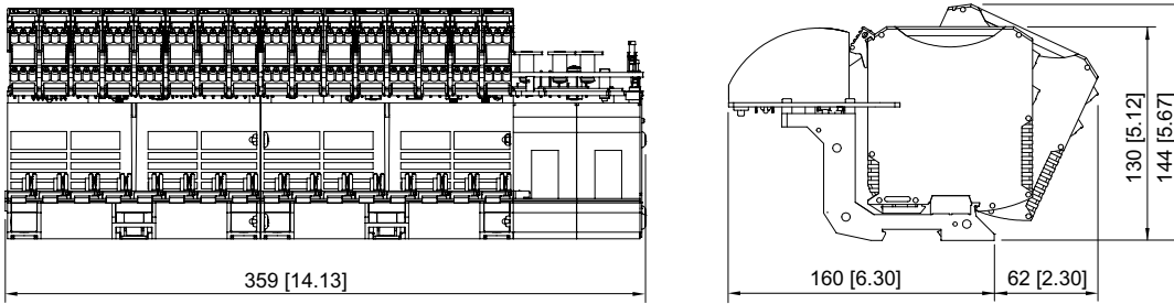
9419/08R bus-Carrier for 16 fieldbus segments
