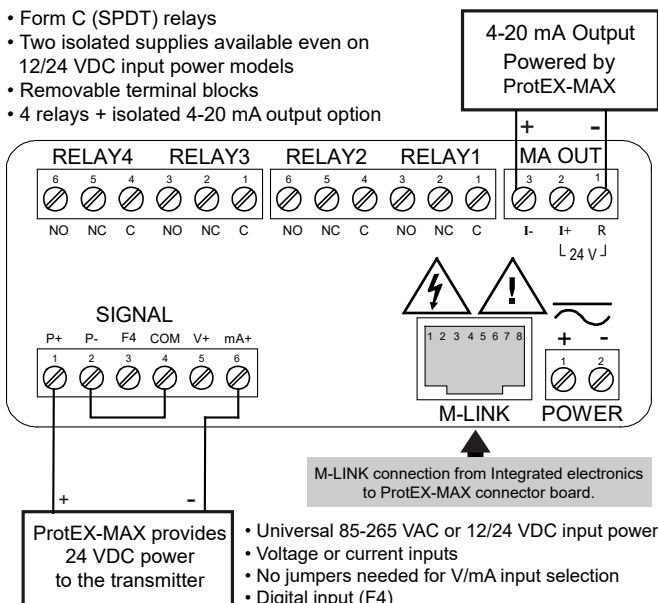
Connections for PD8-6000-6H7 & PD8-6000-7H7
