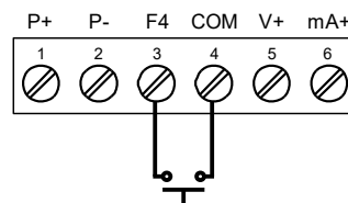
F4 Terminal for Digital Input
