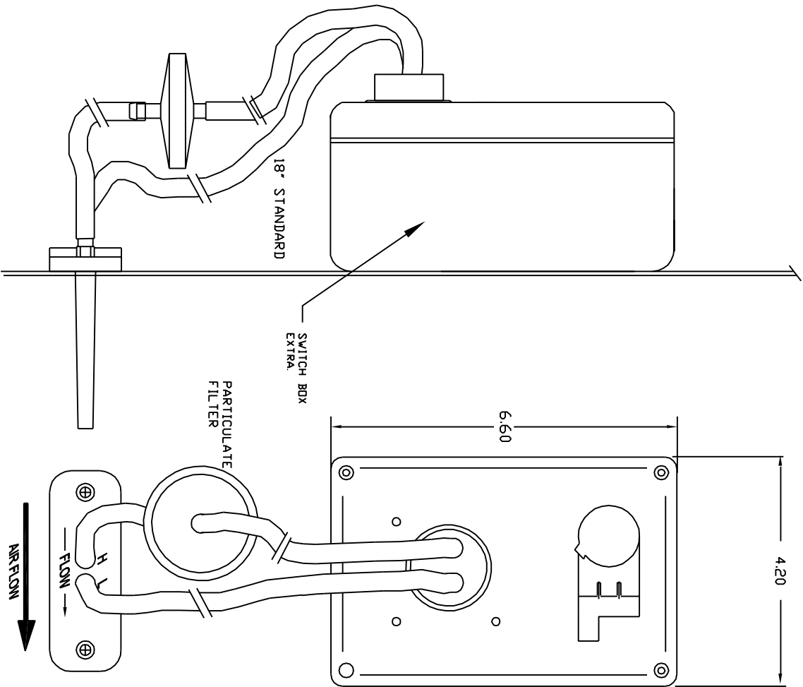
DUCT MOUNTING OPTION
