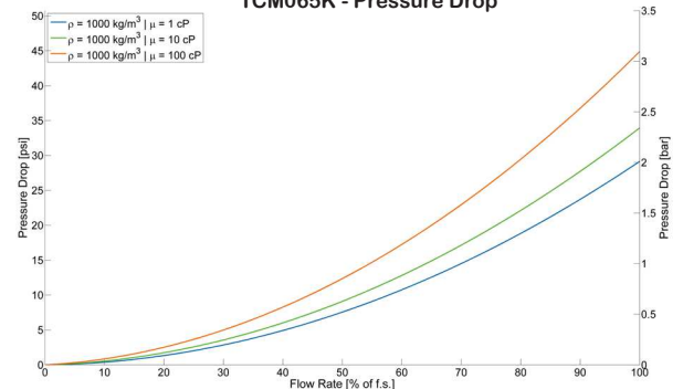
TCM065K - Pressure Drop
