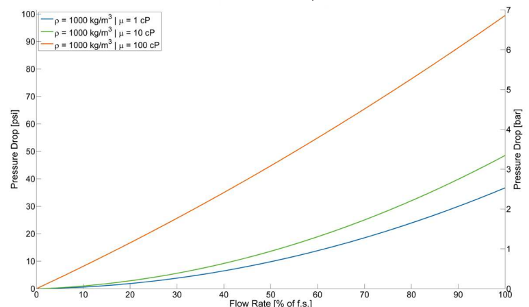
TCM1550 - Pressure Drop
