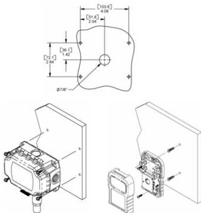
FIGURE 1: Mounting Diagram
