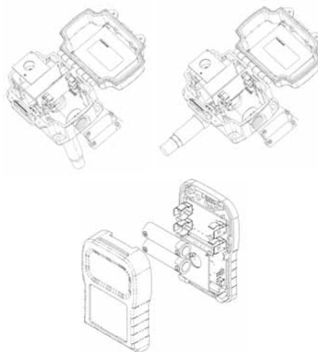
FIGURE 3: Battery Polarity
