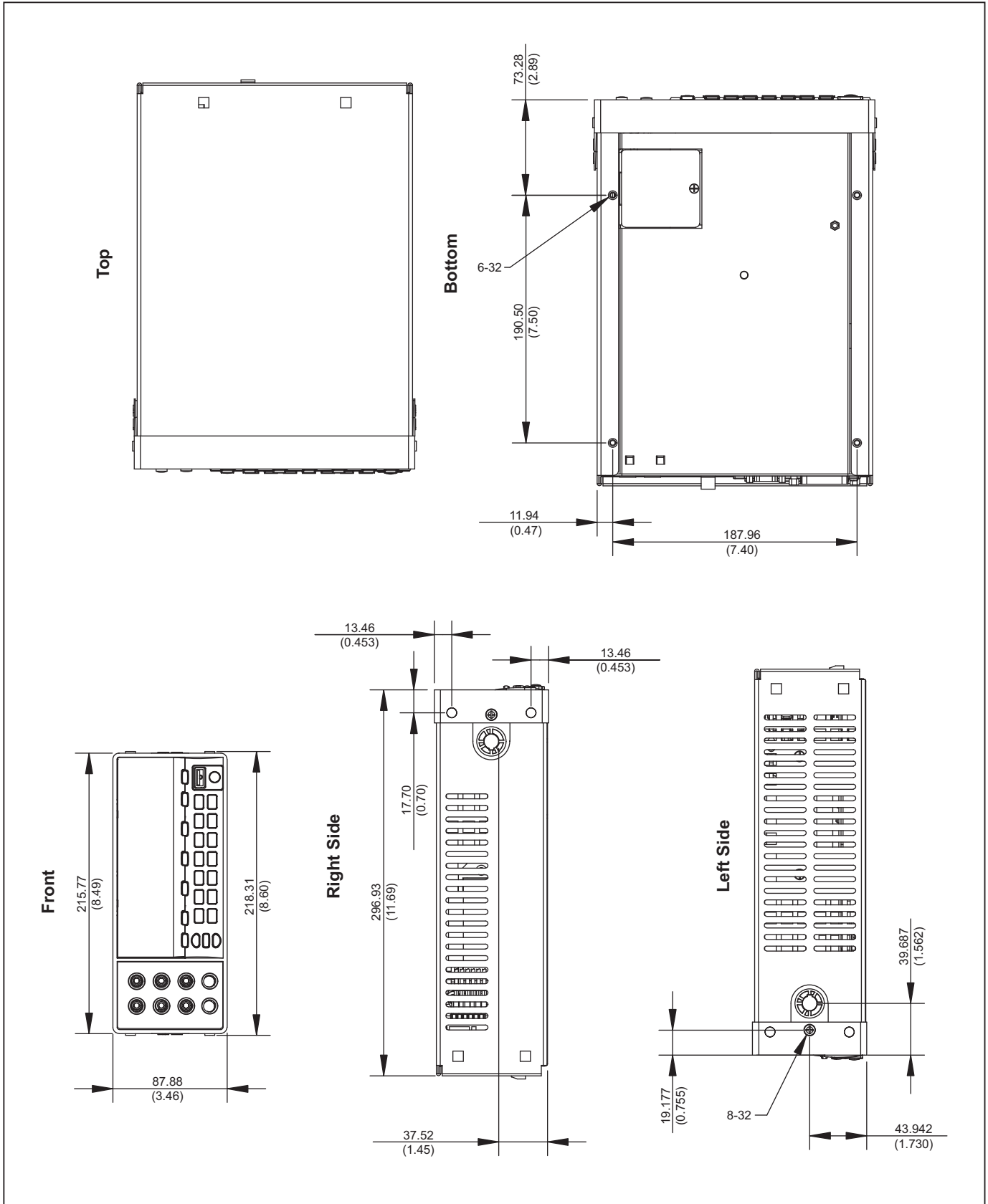
Figure 4. Dimensions
