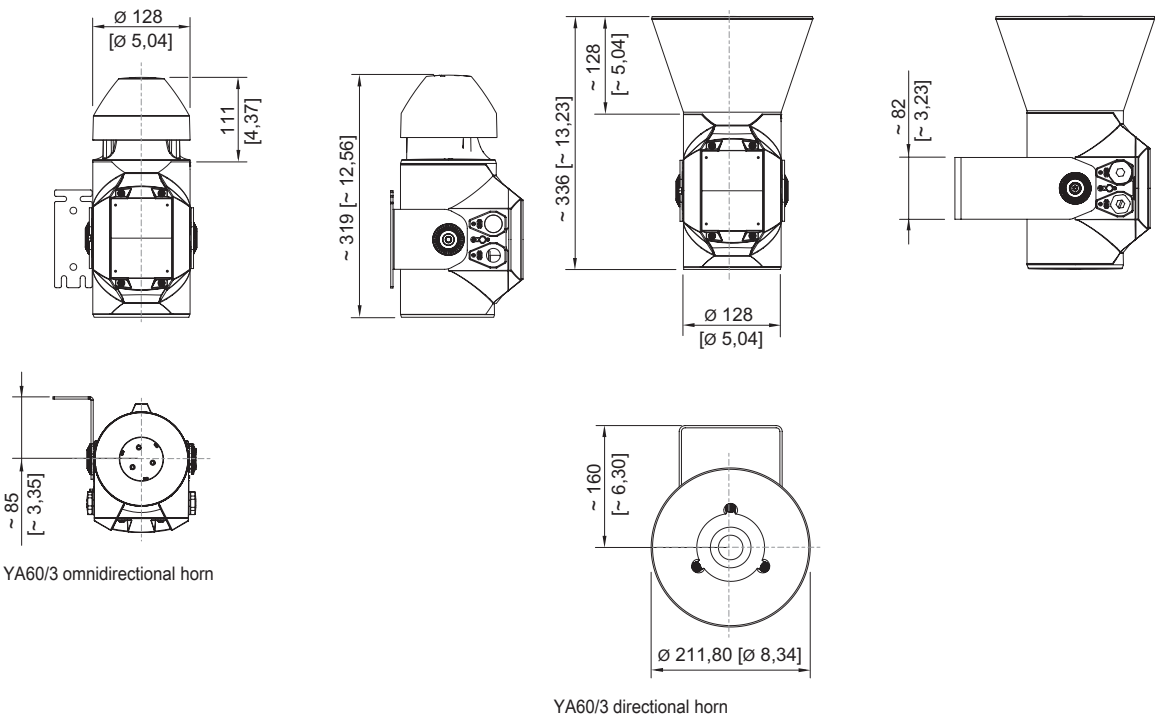
YA60/3 directional horn
